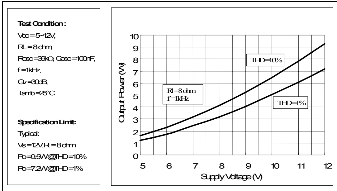
Figure 32. Output power vs supply voltage
