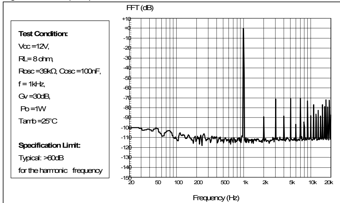
Figure 39. FFT (-60 dB)
